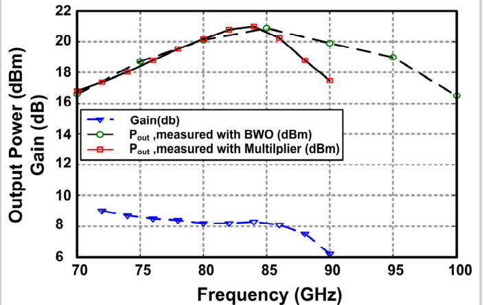
Figure 11.8.6: Measured saturated power and gain versus frequency.
