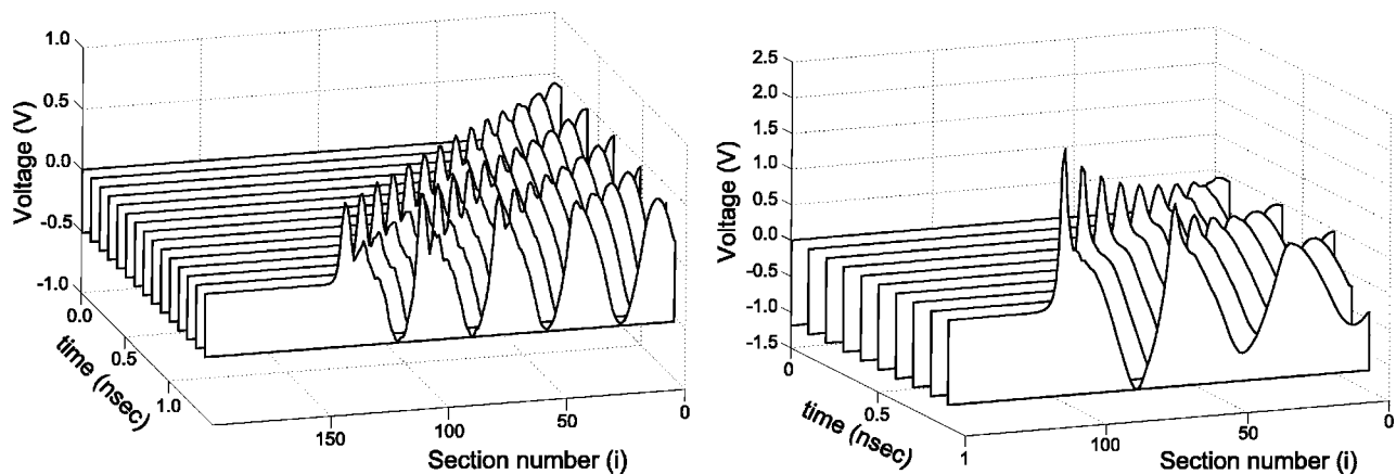
FIG. 3. Voltage V_i vs element number i at various times for the (a) uniform NLT, with b=0.5 , \lambda=0 , and (b) nonuniform NLT, with b=0.25 , \lambda=0.02 . All other parameters are the same as in the linear case. The input frequency is \alpha=5 GHz.
