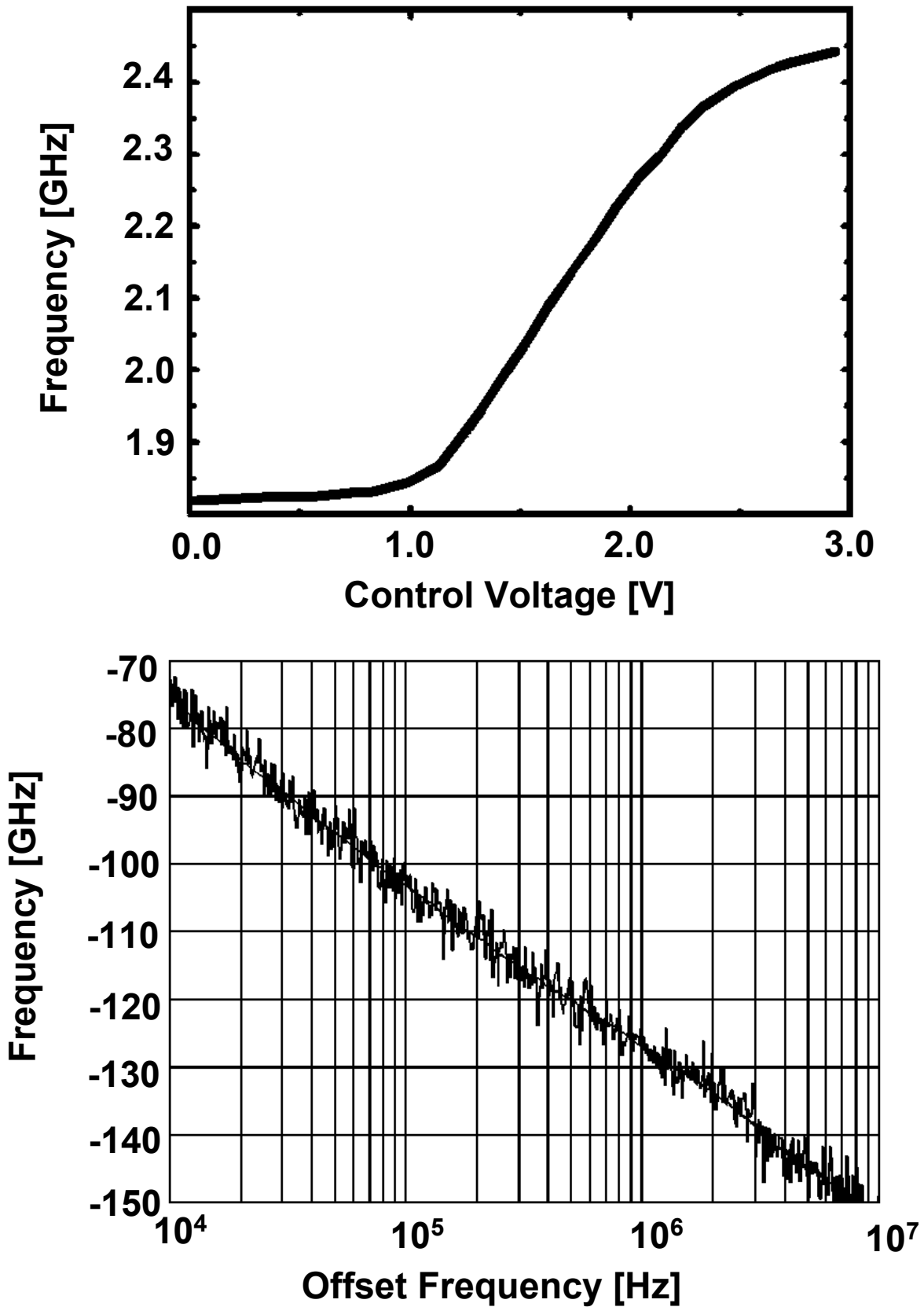
Figure 17.2.5: Measured frequency tuning range of the VCO (b) measured phase noise plot at f_{osc} = 1.8 GHz.
